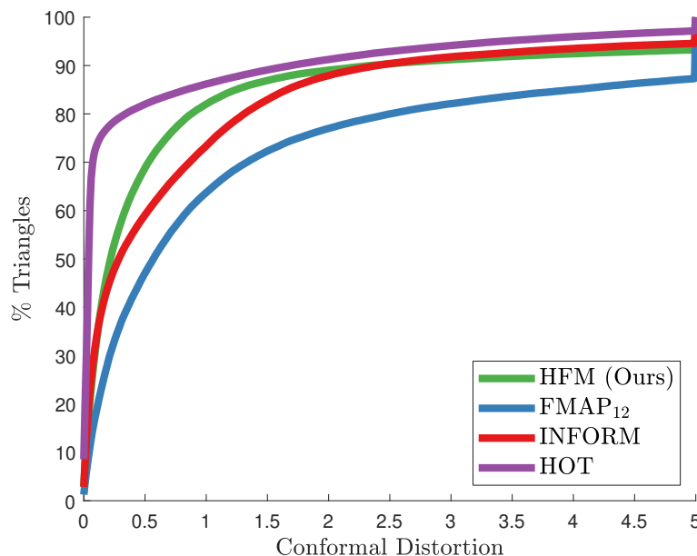
Figure 6.3: Quantitative comparison of the conformal distortion of the maps. We compare our method (HFM), the non hierarchical functional maps scheme FMAPS12 [OBCS + 12], INFORM [NO17] and HOT [AL16]. HOT achieves the best conformal distortion, at a 25 \times higher computational cost, our method is second.
