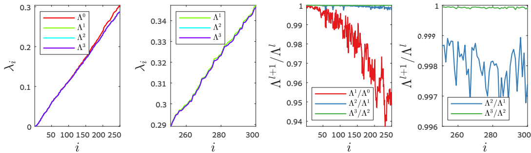
Figure 3.3: (left and center left) The eigenvalues of \mathbb{L}^l at different levels, note the similar trends. (center right and right) The ratio \Lambda^{l+1}/\Lambda^l for the different levels, note that the similarity breaks later for higher levels, and the ratio is very close to 1.
