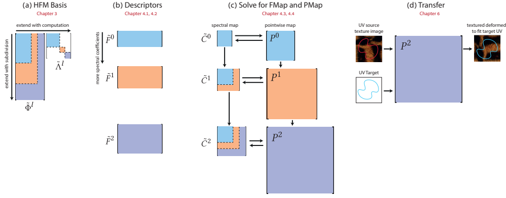
Figure 2.1: An illustration of our pipeline, (a) compute a hierarchical basis, (b) set up linear constraints from spectral descriptors, (c) solve hierarchically for the spectral functional map and the corresponding pointwise map at all levels, and (d) use the final fine pointwise map for texture image and displacement transfer.
