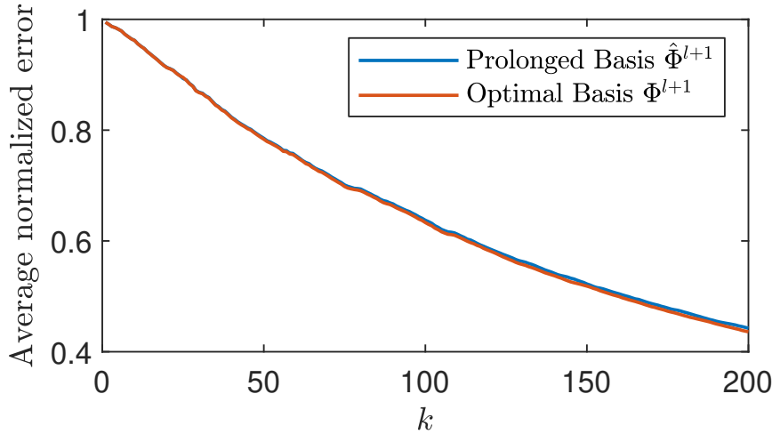
Figure 3.1: Average representation error for 1000 random functions in the image of S^l , normalized by the functions' squared norm, as a function of the number of eigenvectors k . We compare using the prolonged eigenvectors \hat{\Phi}^{l+1} , with the optimal representation error achieved by using \Phi^{l+1} . Note that while the exact eigenfunctions achieve a slightly better representation error for larger k values, the graphs are almost indistinguishable.
