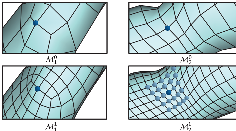
Figure 4.2: Illustration of the hierarchical nearest neighbor search. (top) Two matching vertices at level 0. (bottom) The only candidates considered for a match of a refined vertex of \mathcal{M}_1^1 (bottom left) are the non-zero entries in S_2^0 , in the column that corresponds to the vertex from level 0 (bottom right).
