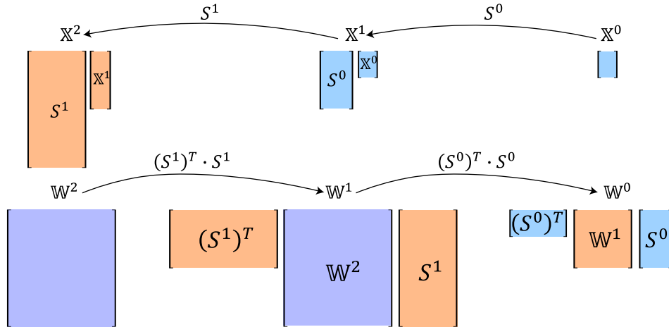
Figure 2.2: An illustration of the construction of the refined geometries (top), and the SEC discrete differential operators (bottom). We map between geometries at the finest subdivision level.
