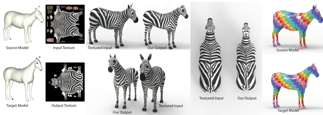
Figure 6.6: Texture transfer of a zebra to a horse. (left to right): input source and target models with corresponding landmarks, input and output texture image, pairs of textured inputs and textured outputs from multiple views, map visualization with checkerboard texture transfer.
