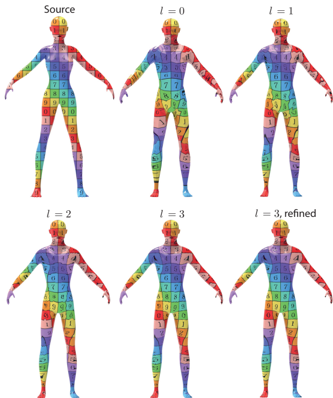
Figure 4.3: Visualization of the map during the hierarchical process. Notice how the map improves as the resolution increases.
