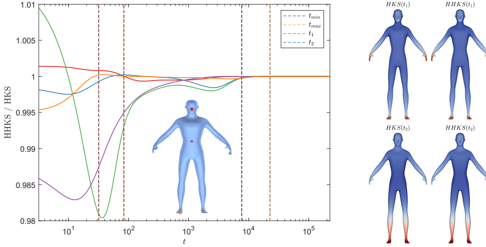
Figure 4.1: Quantitative and qualitative evidence to the Hierarchical HKS approximation quality. (left) The ratio of the HHKS and the HKS for a few vertices as a function of t , (right) the exact and hierarchical HKS for two times t as a function on the mesh. Note that as t increases the error decreases, and that even for small t the error is less than 2 percent, and visually indistinguishable. t_{min} and t_{max} as recommended by [SOG09].
