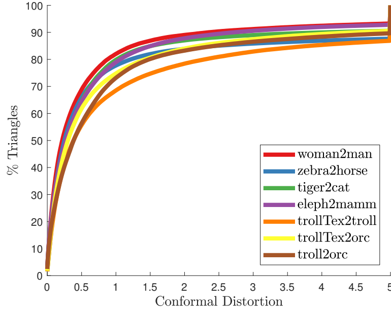
Figure 6.1: Conformal distortion of the maps for all our experiment pairs.
