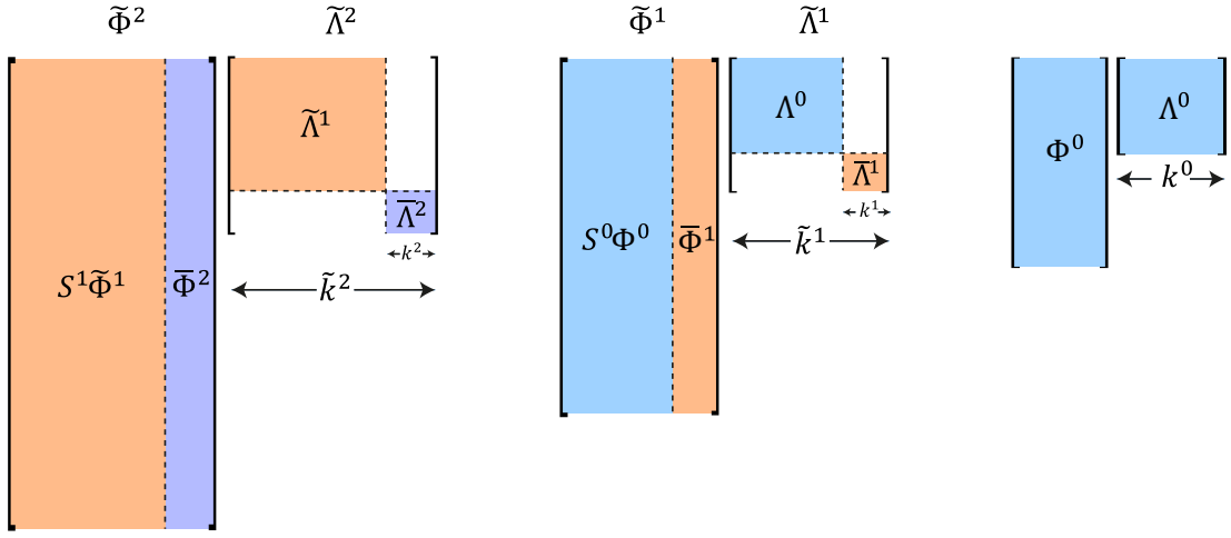
Figure 3.4: An illustration of the hierarchical basis construction from Definition 3.1.4.
