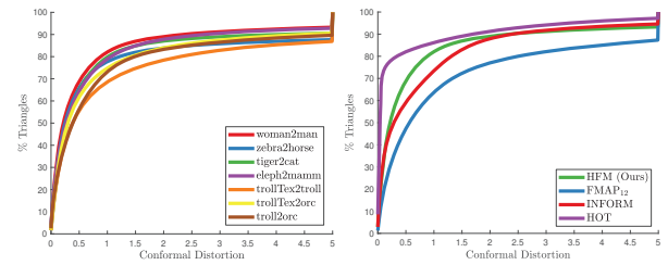
Figure 12: (left) Conformal distortion of the maps for our experiments. (right) Quantitative comparison of the conformal distortion of the maps. We compare our method (HFM), the non hierarchical functional maps scheme FMAPS12 [OBSC* 12], INFORM [NO17] and HOT [AL16]. HOT achieves the best conformal distortion, at a 25 \times higher computational cost, our method is second.
